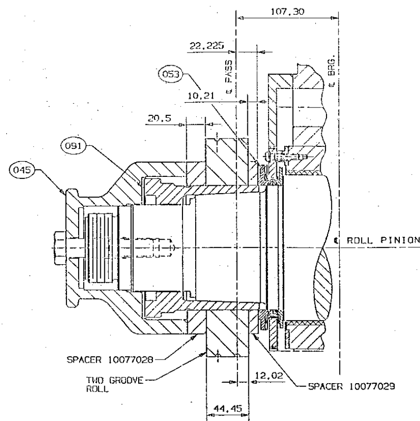
Ⓑ RUNNING COVER ARRANGEMENT FOR TWO GROOVE ROLLS (10077024) NOTE: ALL DIMENSIONS SHOWN ARE NOMINAL.
