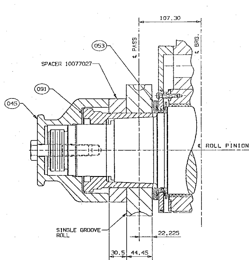
Ⓑ RUNNING COVER ARRANGEMENT FOR SINGLE GROOVE ROLL (10077024) NOTE: ALL DIMENSIONS SHOWN ARE NOMINAL.
