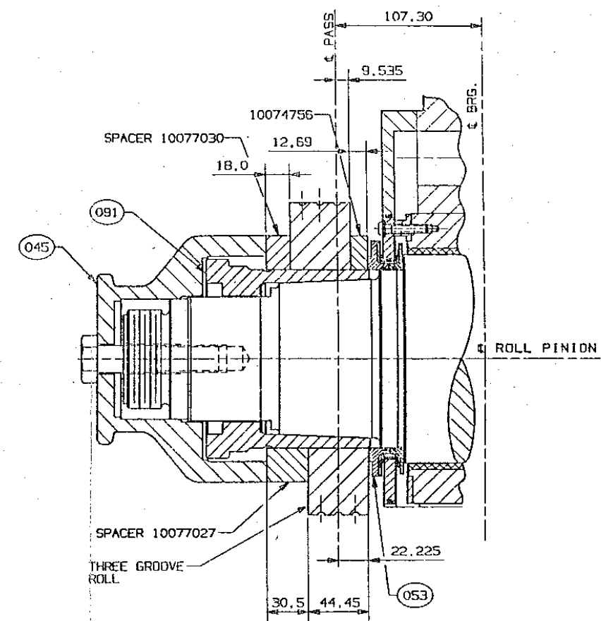
Ⓑ RUNNING COVER ARRANGEMENT FOR THREE GROOVE ROLLS (10077024) NOTE: ALL DIMENSIONS SHOWN ARE NOMINAL.
