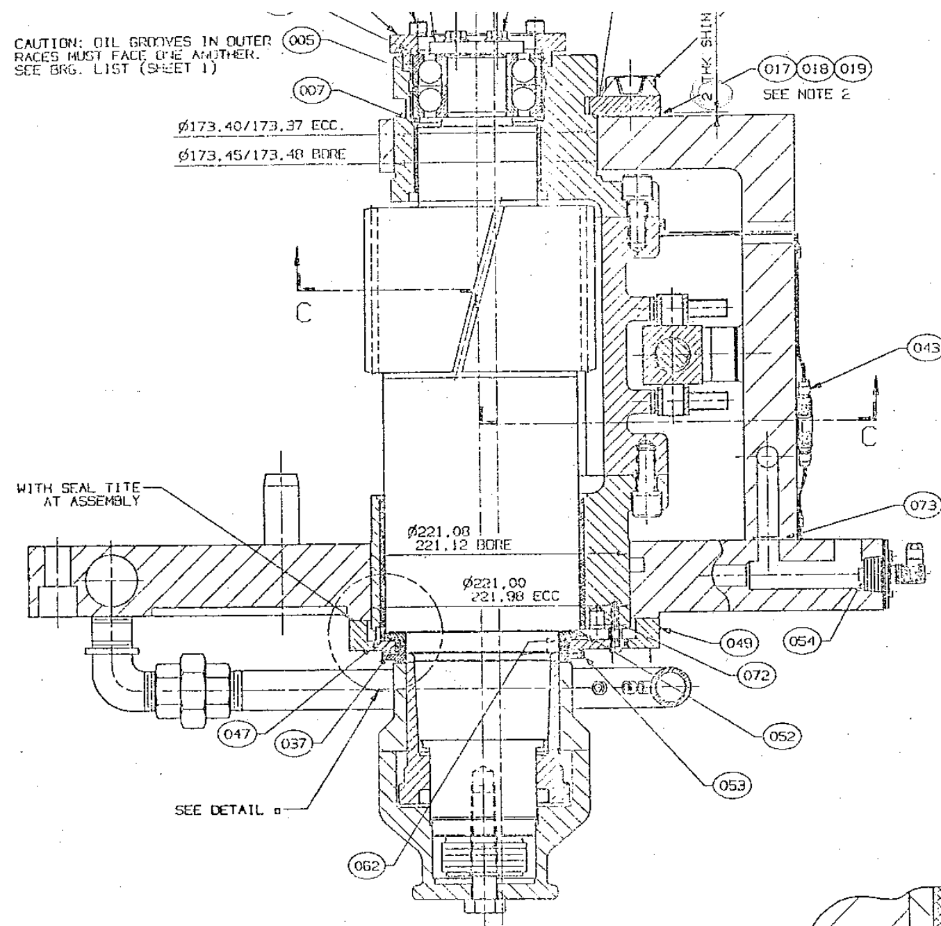
SECTION B-B (SHEET 1)
